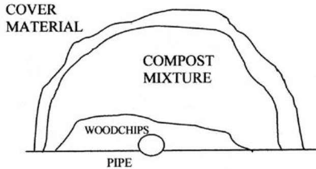
Figure 1. Diagram of a static pile construction with a perforated pipe insert.
